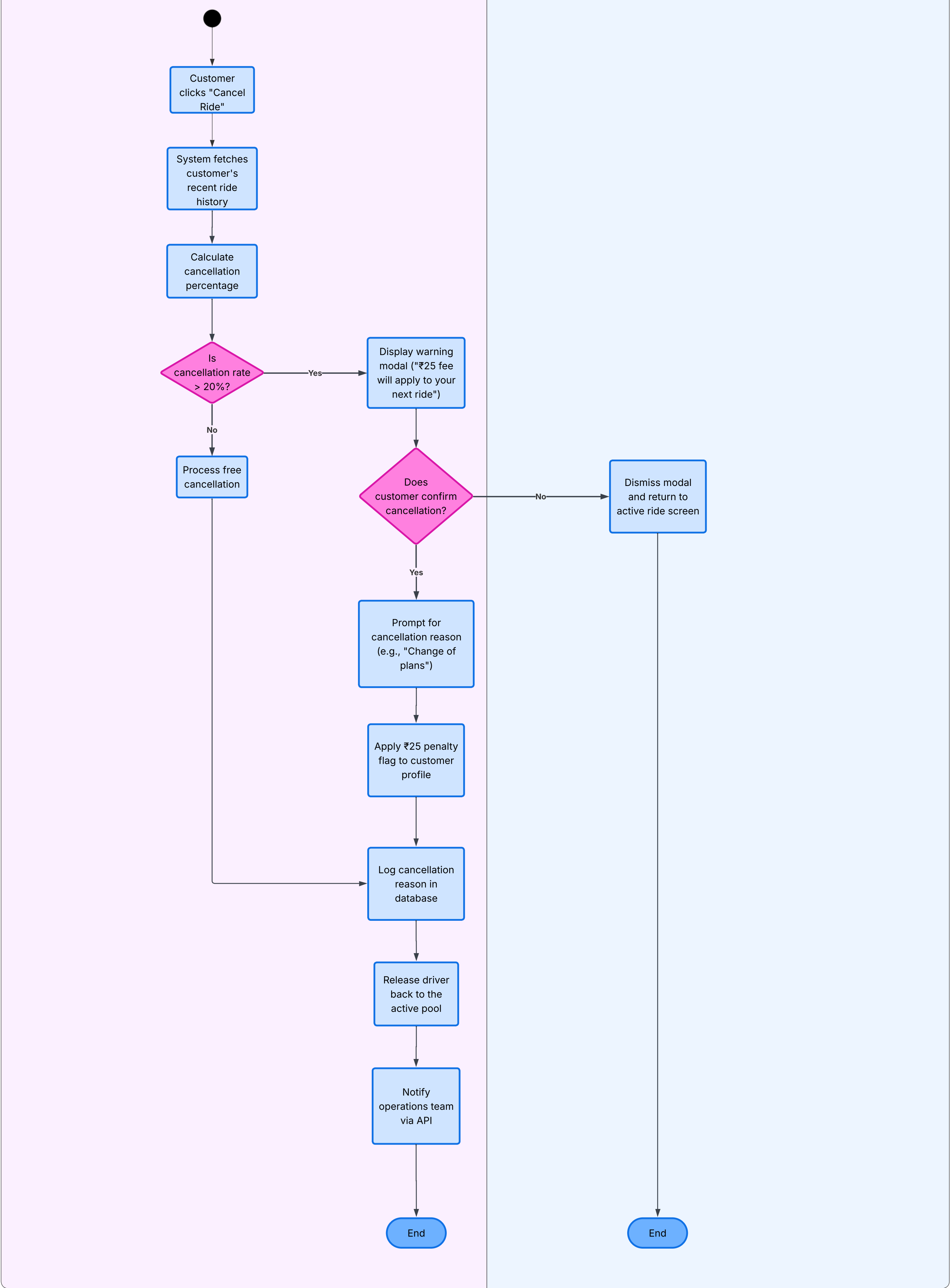
Activity Diagram: OLA Cancellation
